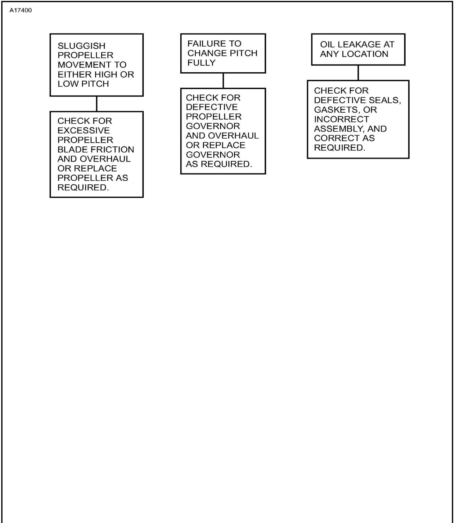
Figure 101 : Sheet 2 : Propeller Troubleshooting Chart
