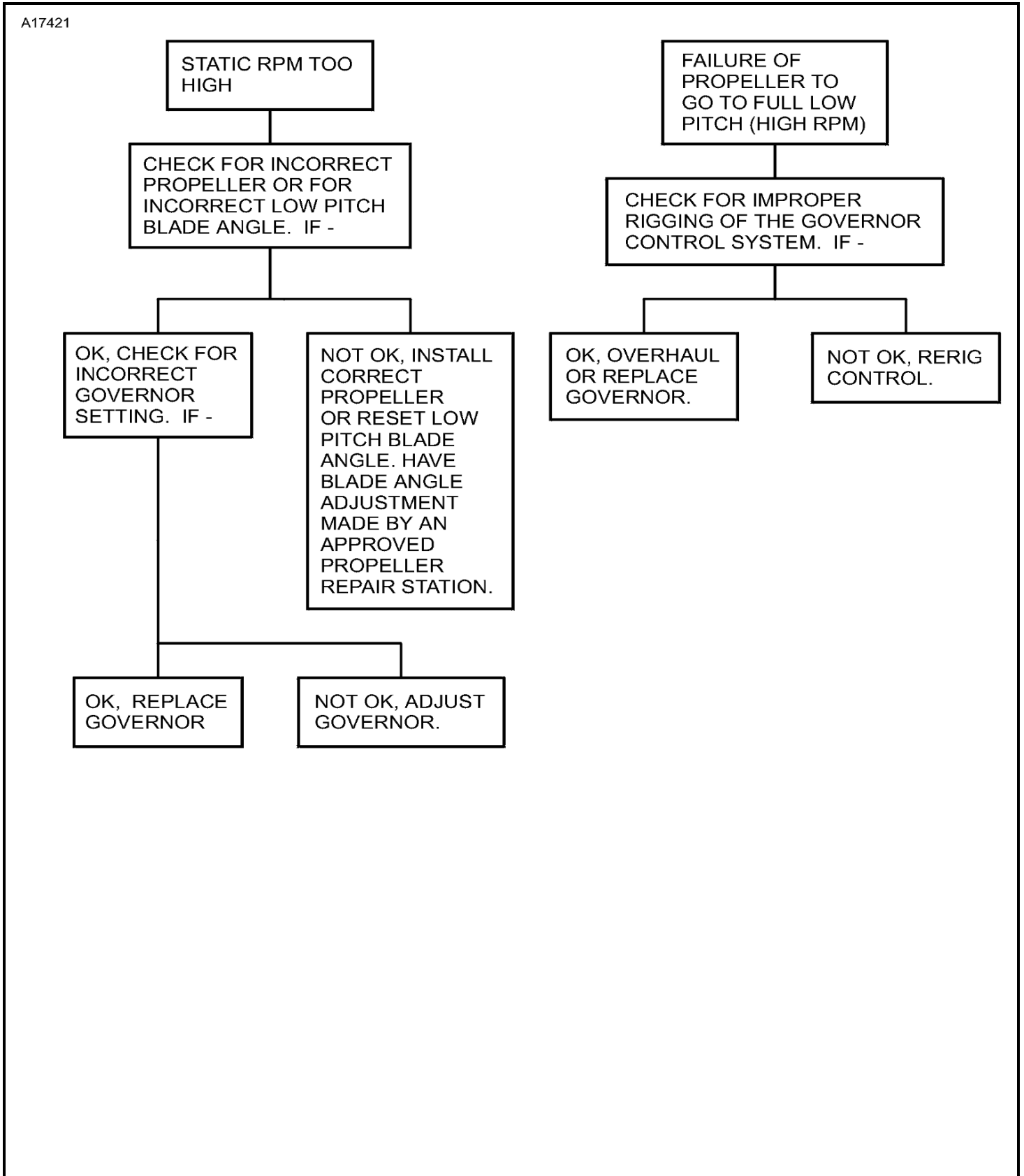
Figure 101 : Sheet 5 : Propeller Troubleshooting Chart
